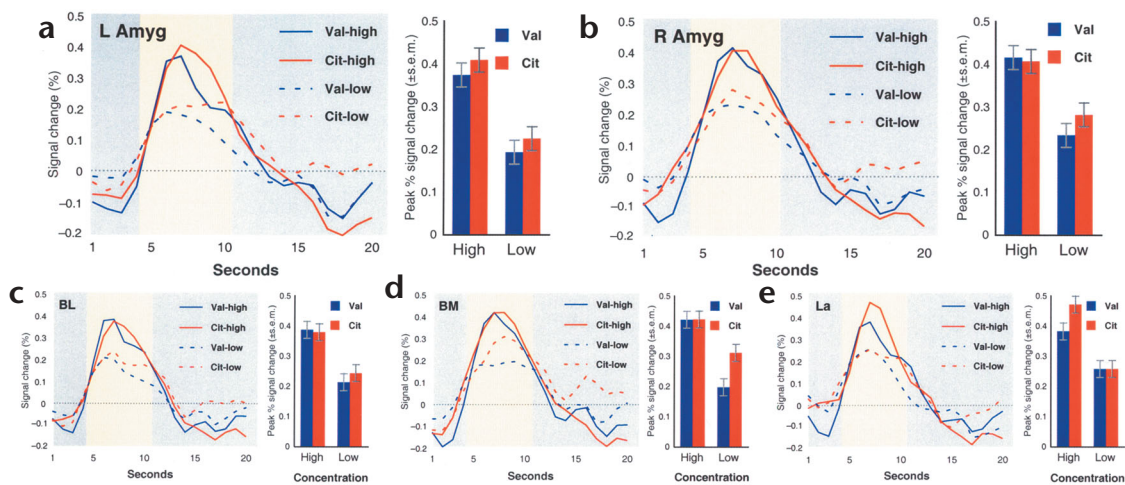
Fig. 3. Time course of amygdala BOLD response. Presented are time course (left-hand graphs) and peak hemodynamic responses (right-hand graphs) to the high and low intensity presentations of valeric and citral in the left (a) and right (b) amygdala. Data also shown for the proposed basolateral (c), basomedial (d) and lateral accessory (e) subdivisions of the amygdala, averaged across both the left and right hemispheres. The time-course ordinate represents percentage signal change, and the abscissa represents time from sniff onset. The peak-response ordinate represents peak percent signal change ( \pm s.e.m.). Mean peak responses are shown from the interval of 4–10 s (cit-low = citral, low intensity; cit-high = citral, high intensity; val-low = valeric, low intensity; val-high = valeric, high intensity).
