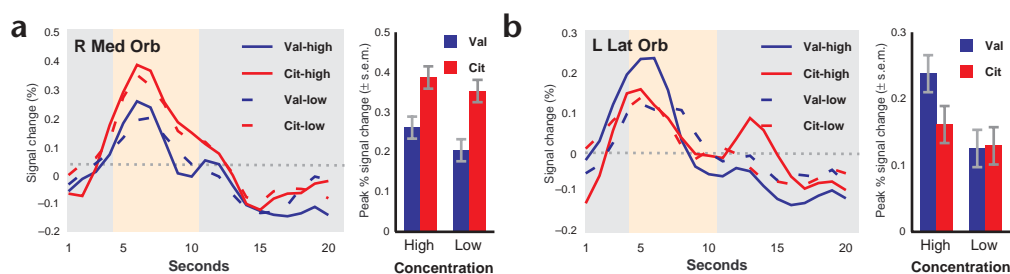
Fig. 4. Time course of orbitofrontal BOLD response. Time course (left-hand graph) and peak hemodynamic response (right-hand graph) to the high and low-intensity presentations of valeric and citral in the right medial (a) and left lateral (b) orbitofrontal cortex. The time-course ordinate represents percent signal change, and the abscissa represents time from sniff onset. The peak response ordinate represents peak percent signal change ( \pm s.e.m.). Mean peak responses are shown from the interval of 4–10 s (cit-low = citral, low intensity; cit-high = citral, high intensity; val-low = valeric, low intensity; val-high = valeric, high intensity).
