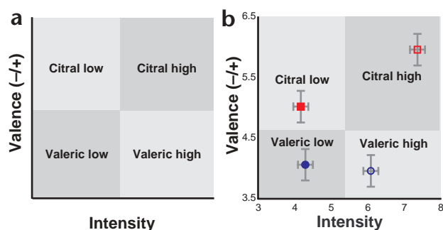
Fig. 1. Ideal and observed odor space. The abscissa represents odor intensity. The ordinate represents odor valence, with increasing pleasantness represented as greater magnitudes. (a) Odor selections were guided by an attempt to construct an affective space whereby odor intensity and valence were manipulated independently. High and low concentrations of the pleasant-smelling citral and unpleasant-smelling valeric acid were psychophysically pre-selected to represent the four critical design quadrants. (b) Subjective intensity and valence estimates obtained after scanning. Horizontal error bars reflect standard error of the mean (s.e.m.) for intensity ratings from 1 (low intensity) to 9 (high intensity) and vertical reflects s.e.m. for valence from 1 (very unpleasant) to 9 (very pleasant). Consistent with the manipulation of odor valence, valeric acid was rated as significantly more unpleasant than citral ( F_{1,15} = 25.30 , P < 0.0001 ). Consistent with the manipulation of odor intensity, high-concentration odors were rated as significantly more intense than low-concentration odors ( F_{1,15} = 78.45 , P < 0.0001 ). Independent manipulation of intensity and valence was achieved for three of the four design quadrants; this was sufficient to separate neural responses to intensity and valence. Low concentrations of citral and valeric acid were equated for intensity ( F_{1,15} = 0.10 , P > 0.75 ), but differed in valence ( F_{1,15} = 6.46 , P < 0.02 ); high and low concentrations of valeric differed significantly in intensity ( F_{1,15} = 20.31 , P < 0.0004 ), but not in valence ( F_{1,15} = 0.08 , P > 0.78 ). High concentrations of citral were rated as more intense ( F_{1,15} = 10.25 , P < 0.007 ) than high concentrations of valeric, and more pleasant ( F_{1,15} = 7.68 , P < 0.01 ) than low citral. Consistent with their relative independence, there was no significant association between individuals' estimations of odor intensity and valence for both odorants (valeric, r = -0.19 , P > 0.27 ; citral, r = 0.29 , P > 0.11 ).
