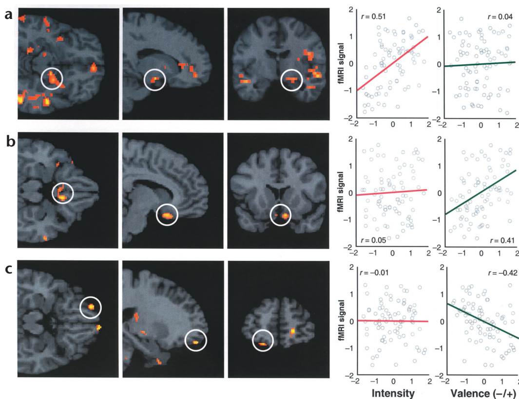
Fig. 5. Functional regions of interest (fROI) defined by their correlation with individual differences either in the evaluation of intensity, pleasantness or unpleasantness of the four odor conditions and clean air. Scatter plots depict the degree of association between individuals' fROI signal and valence and intensity evaluations (depicted as circles in standardized units). The ordinate represents fMRI signal, and the abscissa represents either the evaluation of odor intensity or valence for each stimulus condition for each participant. (a) A region in the right hemisphere extending from the dorsal amygdala into the piriform cortex was correlated with the evaluation of intensity but not valence. (b) A bilateral subcallosal gyrus activation extending into the posteromedial orbitofrontal cortex was correlated with the evaluation of pleasantness but not intensity. (c) Left anterior lateral and right anterior medial orbital cortical activations were correlated with the evaluation of unpleasantness but not intensity.
