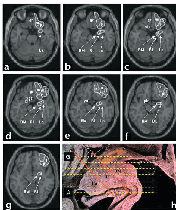
Fig. 2. Region of interest (ROI) analysis. Anatomical subdivisions of the amygdala and orbitofrontal cortex were outlined for analysis. Shown here are seven slices of the acquisition that typically contained the ROIs, from the most ventral (a) to dorsal (g). ROIs were drawn bilaterally (shown unilaterally here) on each participant's anatomical scan (m, medial orbitofrontal; p, posterior orbitofrontal; a, anterior orbitofrontal; BM, basomedial amygdala; BL, basolateral amygdala; La, lateral accessory amygdala). The amygdaloid complex is made up of numerous structures, but these are not separable on the MR image. Thus, we opted for a crude segmentation into these three amygdala subregions based on a detailed atlas 24 . (h) As can be seen from the cytoarchitecture, there is a coarse inferior-superior organization to the amygdala in oblique bands (red lines), with the La being most inferior, the BM most superior and the BL in-between. Overlaid on the coronal image (from ref. 24) are approximated slices of the current acquisition (yellow dotted lines). As the temporal portion of piriform cortex cannot be distinguished from the anterior end of the piriform on the MR image, the amygdala ROI was drawn conservatively at this point (slices d-f).
